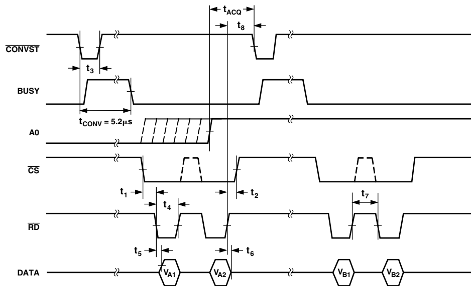
Figure 1. Timing Diagram
